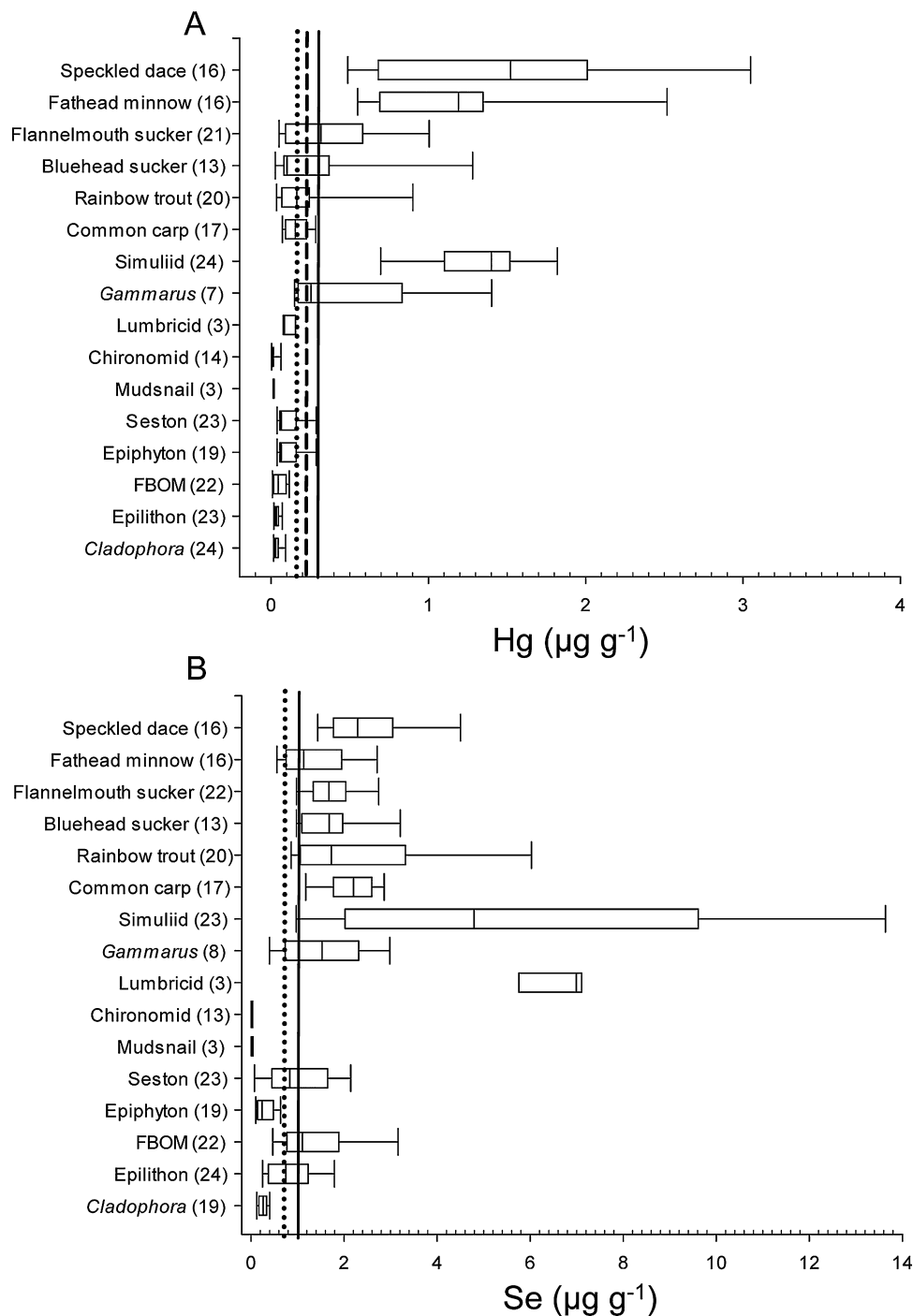
Figure 5. Concentrations ( \mu\text{g g}^{-1} wet wt) of Hg ( A ) and Se ( B ) in organic matter and consumers among all sites sampled in the Colorado River, Grand Canyon (AZ, USA). Numbers in parentheses indicate number of replicates analyzed for each component. Lines within the boxes are the median, and horizontal whiskers indicate the 90th and 10th percentiles. Vertical lines in the Hg plot are risk thresholds for piscivorous mammals ( 0.16 \mu\text{g g}^{-1} ; dotted line), fish ( 0.2 \mu\text{g g}^{-1} ; dashed line), and humans ( 0.3 \mu\text{g g}^{-1} ; solid line). The whole-body-corrected risk threshold for kingfisher ( 0.04 \mu\text{g g}^{-1} ) is not included in the figure because all fishes exceeded this threshold. Vertical lines in the Se plot are risk thresholds for piscivorous wildlife ( 0.75 \mu\text{g g}^{-1} ; dotted line) and larval fish ( 1.0 \mu\text{g g}^{-1} ; solid line). FBOM = fine benthic organic matter.
