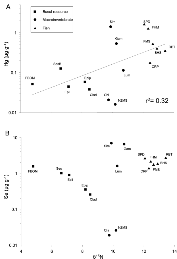
Figure 4. Concentrations ( \mu\text{g g}^{-1} wet wt) of Hg ( A ) and Se ( B ) relative to \delta^{15}\text{N} for the Colorado River food web in Grand Canyon (AZ, USA). Model regression in ( A ) is: \log_{10}\text{Hg} = 0.147(\delta^{15}\text{N}) - 2.259 . BHS = bluehead sucker; Chi = chironomid; Clad = Chladophora ; CRP = common carp; Epil = epilithon; Epip = epiphyton; FBOM = fine benthic organic matter; FHM = fathead minnow; FMS = flannemouth sucker; Gam = Gammarus ; Se = seston; Lum = lumbricid; NZMS = New Zealand mudsnail; RBT = rainbow trout; Sim = simuliid; SPD = speckled dace.
