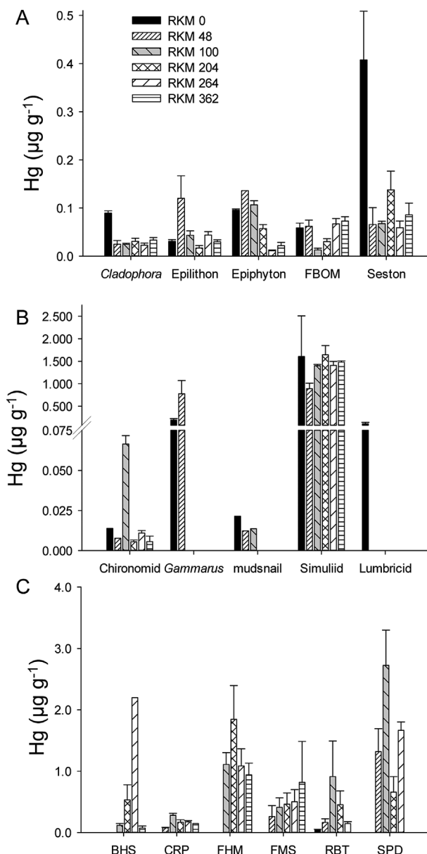
Figure 2. Mercury concentration ( \mu\text{g g}^{-1} wet wt) in (A) basal organic matter resources, (B) invertebrates, and (C) fishes for 6 sites in the Colorado River in Grand Canyon (AZ, USA). Bars show standard error ( n=3-4 samples per site). Rainbow trout was the only species collected at RKM0. Missing bars indicate that no samples of that type were collected at a particular site. RKM = river kilometer; BHS = bluehead sucker; CRP = common carp; FHM = fathead minnow; FMS = flannelmouth sucker; RBT = rainbow trout; SPD = speckled dace.
